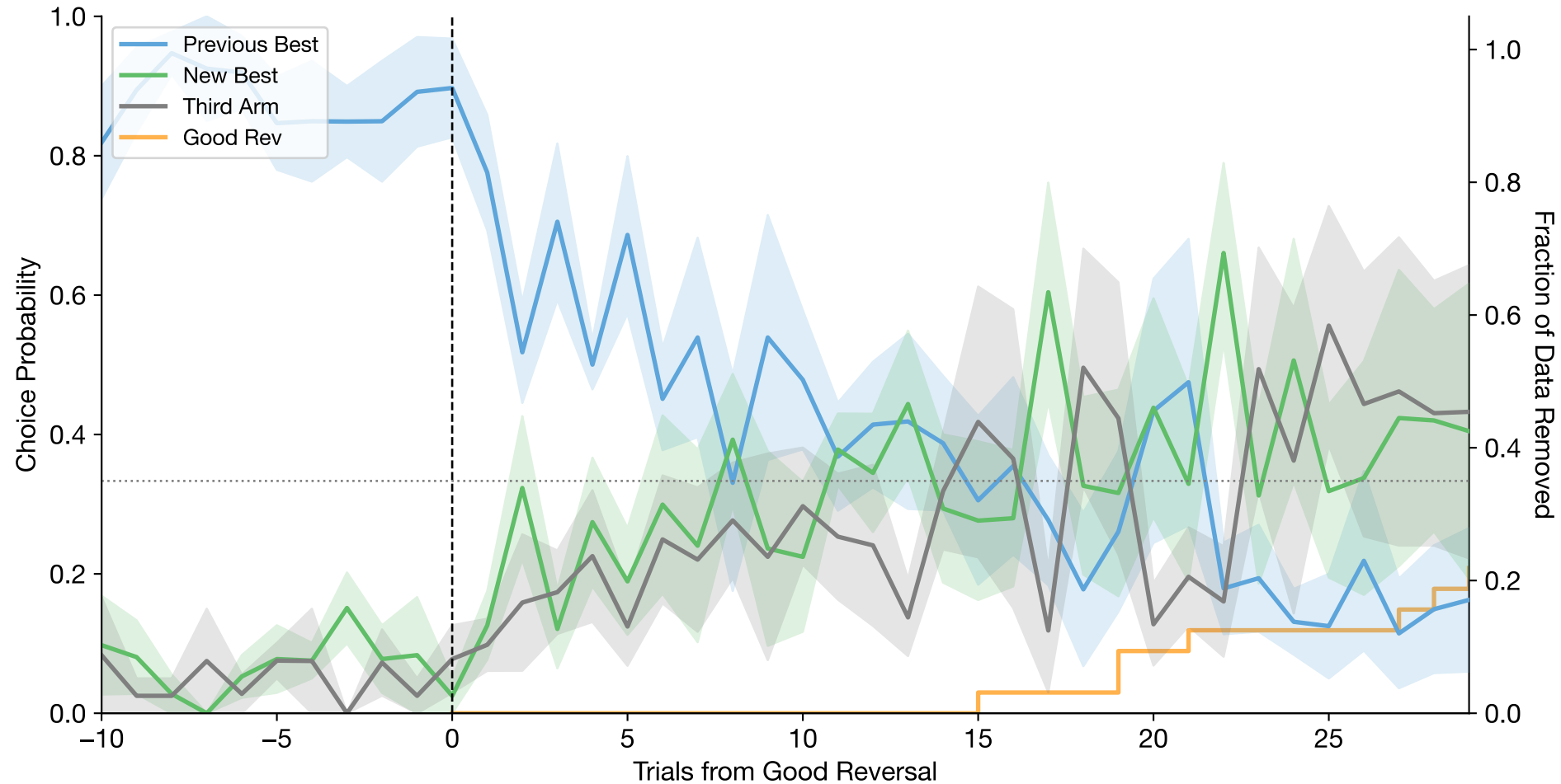
Good Reversal-Aligned Choices (mean \pm se across subjects | n=4 subjects, n=32 reversals)
